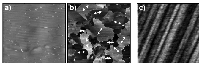
Figure 2. (a) 50 \times 50 \mu\text{m}^2 AFM topography image of a red poly( I ) monolayer. (b) simultaneous friction image. The friction image reveals the different domains. White arrows indicate the domain orientation. (c) A separate 500 \times 500 \text{nm}^2 AFM topography image of a single domain. The striations are indicative of the backbone orientation.
