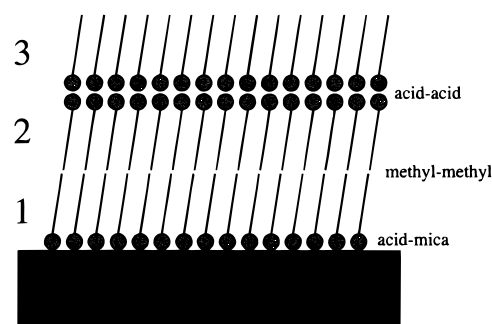
Figure 2. Trilayer packing of PCDA molecules. The circles represent the COOH headgroups which are expected to hydrogen bond to the mica substrate (mica–layer 1 interface) and each other (layer 2–layer 3 interface). Between layers 1 and 2 is a \text{CH}_3 – \text{CH}_3 interface that is less strongly bonded through van der Waals' forces.
