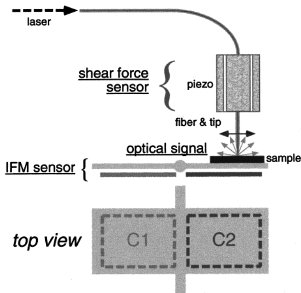
Figure 3. Schematic diagram of the NSOM/IFM instrument. The NSOM fiber is brought into contact with a sample resting on an IFM sensor. The sensor measures the attractive and repulsive normal forces between the tip and sample by maintaining an electrostatic balance of two capacitances C_1 and C_2 , formed by the common plate and identical gold pads fixed on a glass substrate (not shown). Light is launched into the fiber and excites sample fluorescence in the near field. Light is collected in the far field above the sample by an objective (not shown).
