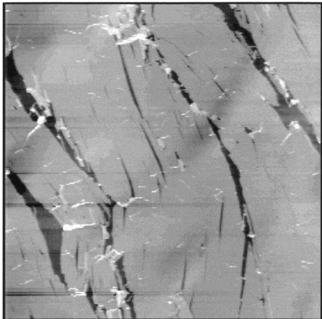
Figure 5. Topographic AFM image ( 50 \times 50 \mu\text{m}^2 ) of fully red PCDA. The sample shows high coverage, with roughly parallel cracks. The cracks are oriented along the polymer backbone direction.
