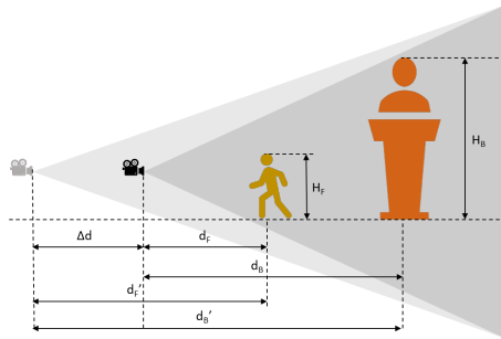
Figure 5.6(a): Geometry of Dolly Zoom
